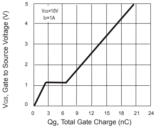
Figure 9. Gate Charge
