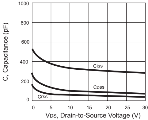
Figure 3. Capacitance
