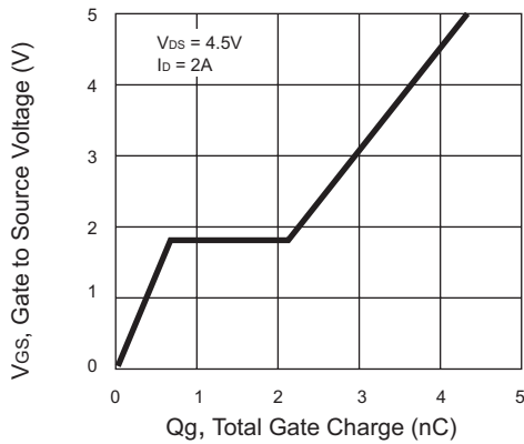
Figure 9. Gate Charge
